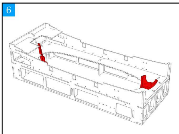
Install keel in the dock
