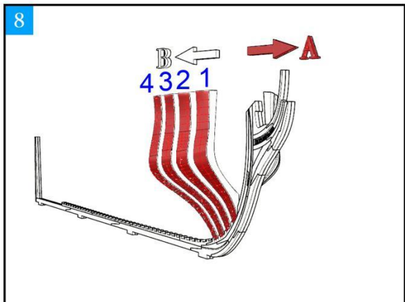
Install ribs 1-4#
