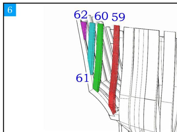
Pay attention to the spacing between ribs 59# and 60#
