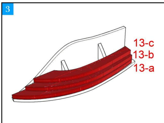
Place the polished internal ribs onto the template
