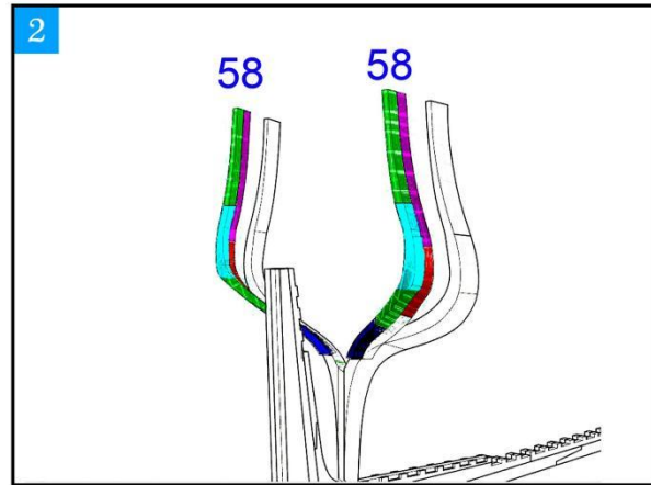
Building 58# ribs
