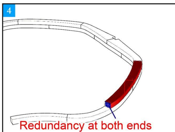
Install the upper ribs gradually
